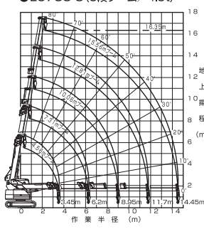
●LC755-3(5段ブーム／4.9t)
